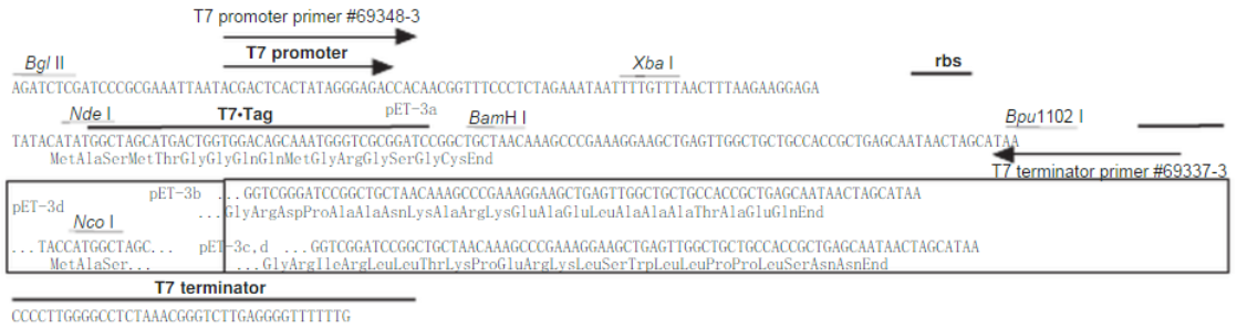
pET-3a-d cloning/expression region
