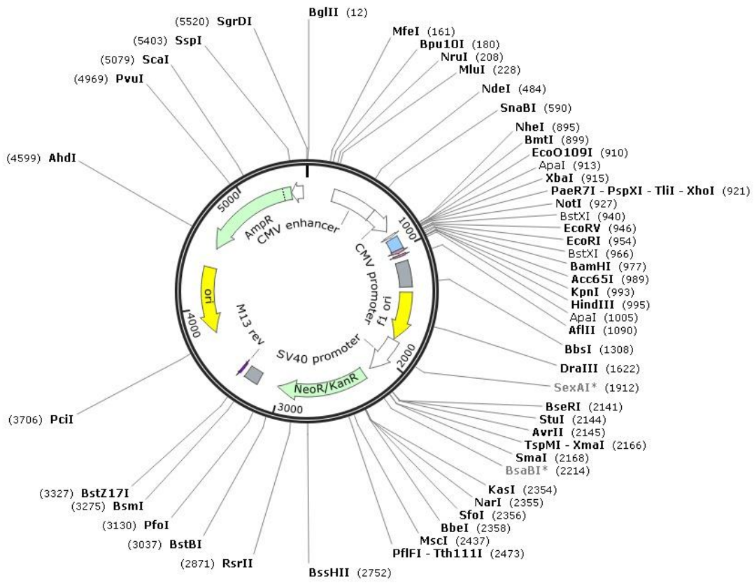
pcDNA TM 3.1/myc-His(-) A 5522 bp
